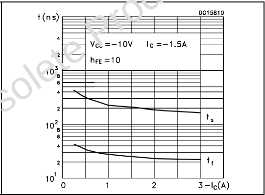
Figure 10. Switching time resistive load Figure 11. Switching time resistive load
